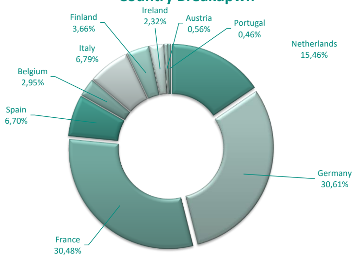
Country Breakdown
